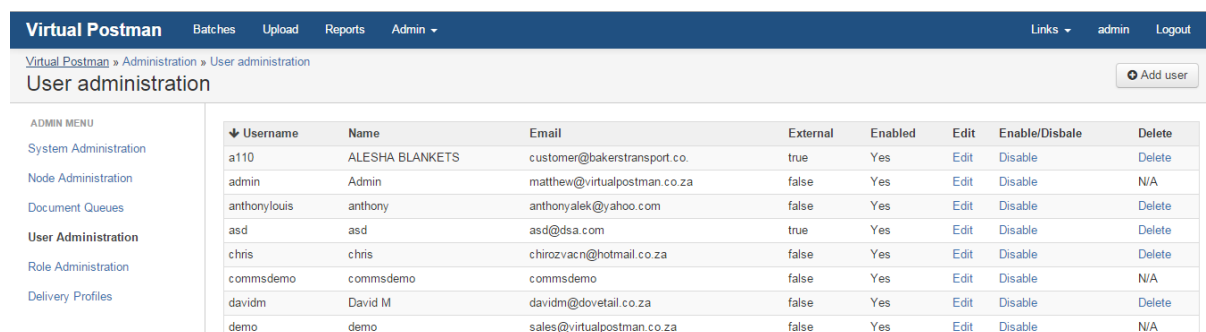
Figure 9.1. Adding Users
